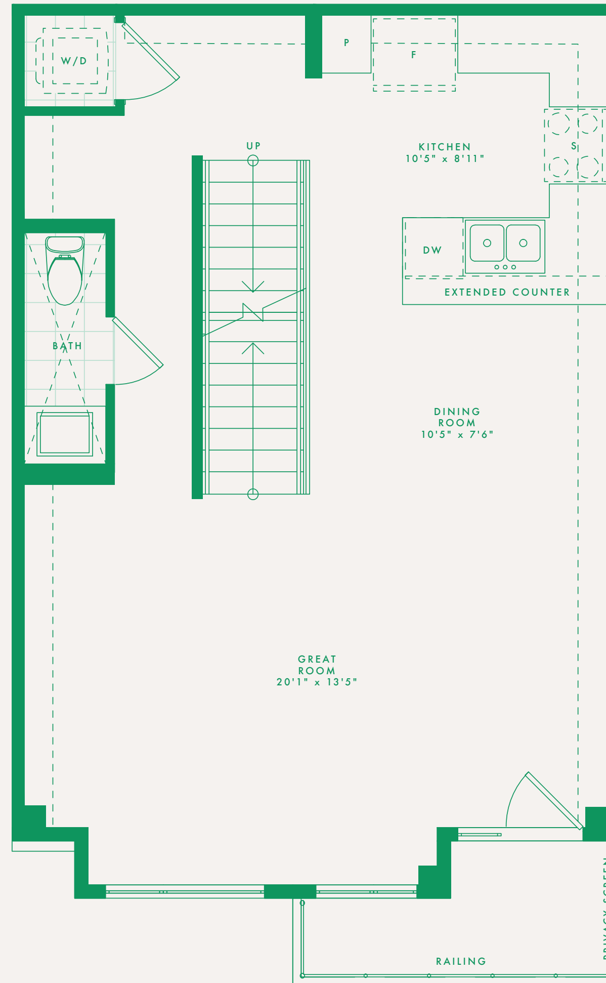
MAIN LEVEL
