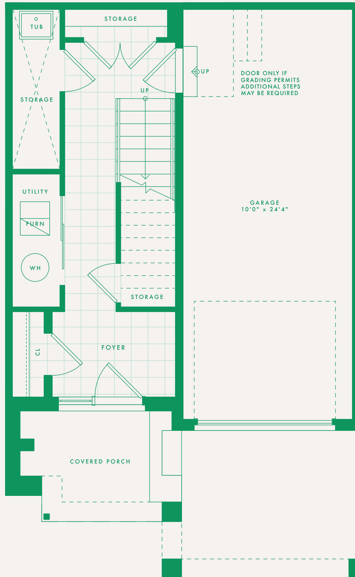
LOWER LEVEL
